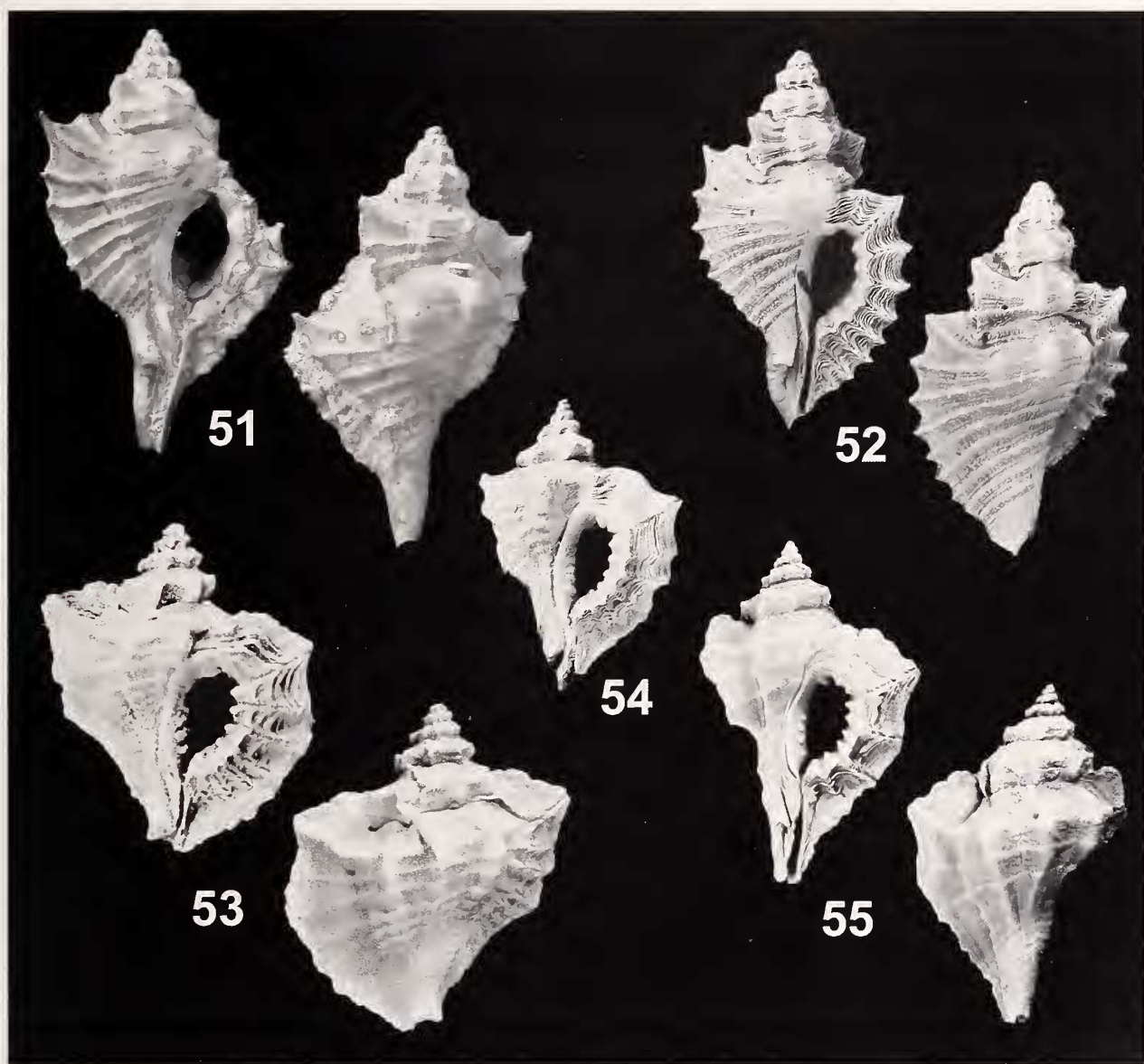
Figures 51–55. Eupleura species. Figure 51. Eupleura olssoni Vokes, 1989. USNM 643957 (Paratype B); locality: Telembi, Río Cayapas, Ecuador; Late Miocene, Angostura Formation; height 27.6 mm, diameter 18.2 mm. Figure 52. Eupleura prenitida Vokes, 1989. USNM 445390 (Holotype); locality: hill-slope on east side of road from Boyd-Roosevelt Highway to Refinería Panama, S. A., about 0.5 km north of junction, just east of Cativá, Prov. of Colón, Panama; Late Miocene, Gatun Formation (= TU 958); height 31.1 mm, diameter 17.7 mm (Photographs courtesy of Emily Vokes). Figures 53–55. Eupleura paroudia Herbert, sp. nov. Figure 53. UF 91974 (Holotype); locality: Roadcut, pipeline cut, and quarry on Mexico Highway 180, 23 km east of junction with side road into Coatzacoalcos, Veracruz, Mexico; Early to middle Pliocene, Agueguexquite Formation (= TU 638); height 19.7 mm, diameter 16.3 mm. Figure 54. UCMP 198994 (Paratype B); locality: Same as Figure 53; height 18.0 mm, diameter 14.2 mm. Figure 55. UF 91972 (Paratype A); locality: Same as Figure 53; height 21.5 mm, diameter 14.0 mm.
